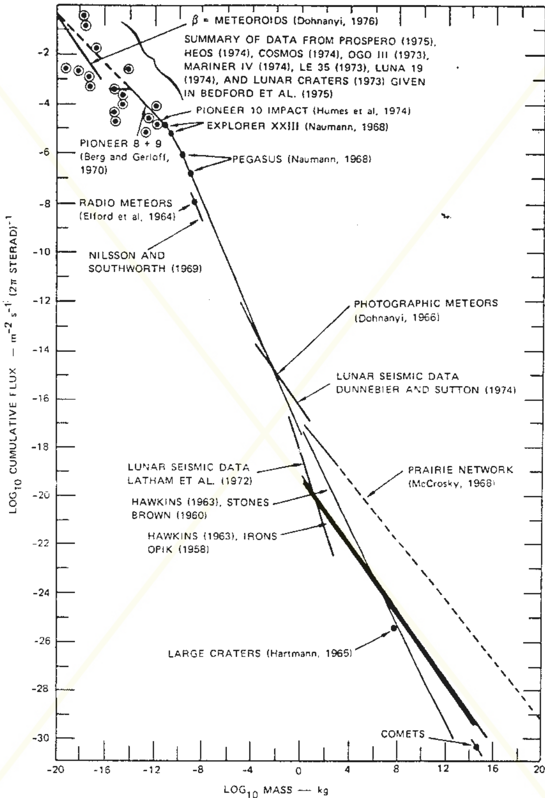
FIGURE 1 METEOROID FLUX DISTRIBUTION (U)
