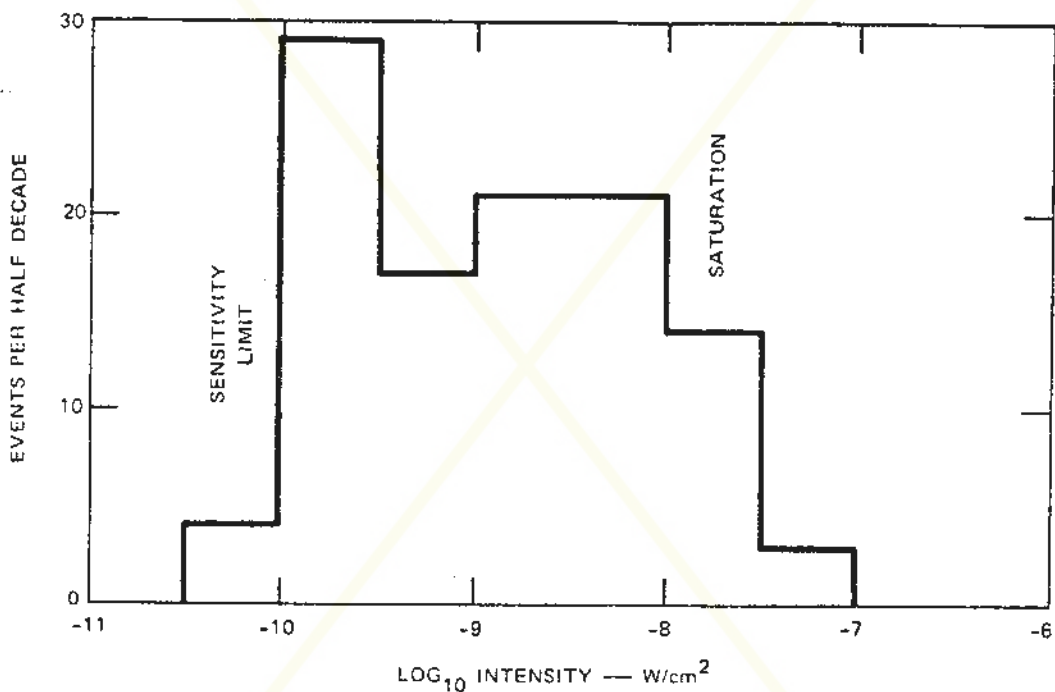
FIGURE 9 DISTRIBUTION OF INTENSITY OF PIONEER 10 EVENTS (U)
