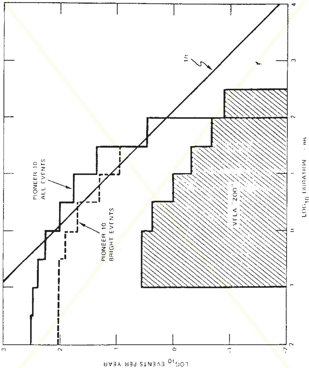
FIGURE 13 CUMULATIVE DURATION DISTRIBUTIONS FOR PIONEER 10 AND THE VELA ZOO (U)
