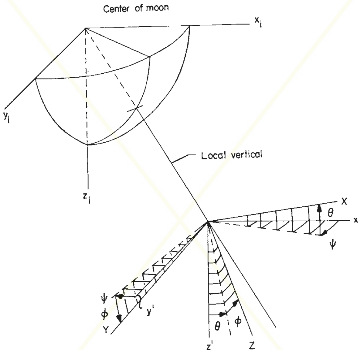
(a) Inertial and vehicle axes systems showing positive rotations and linear displacements of vehicle.
