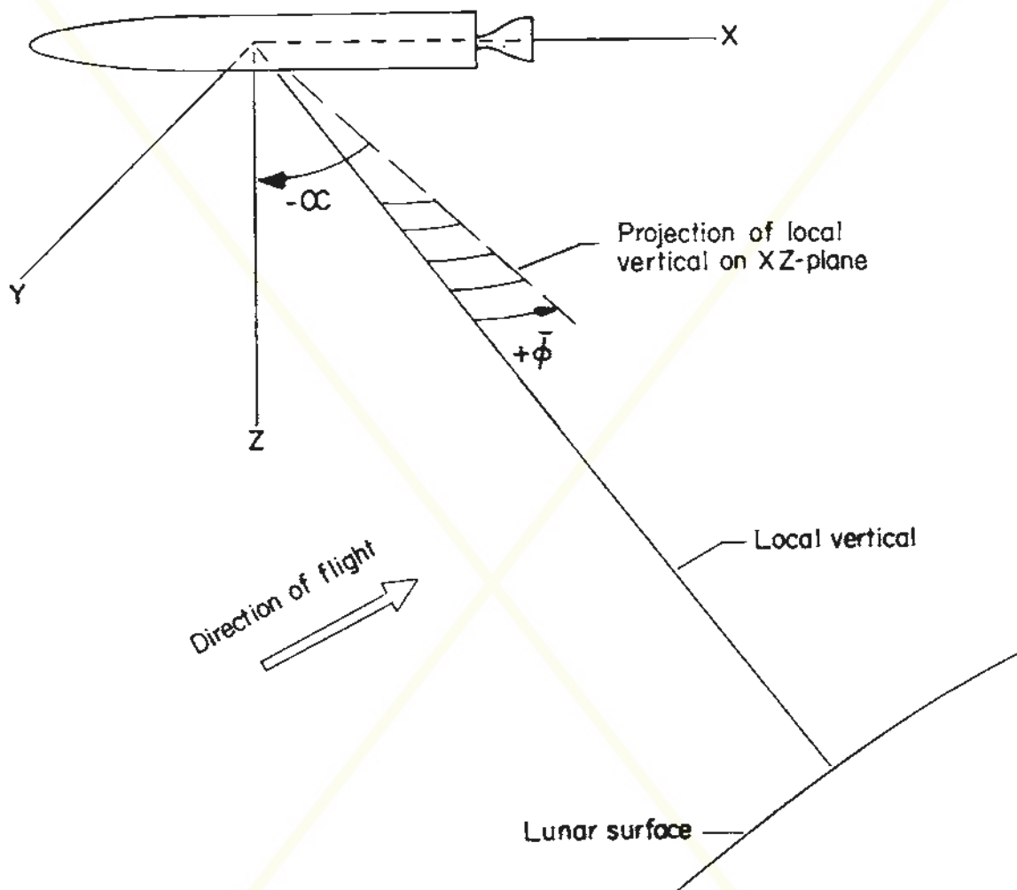
(b) Vehicle attitude angles \alpha and \phi and vehicle orientation relative to body-axis system.
