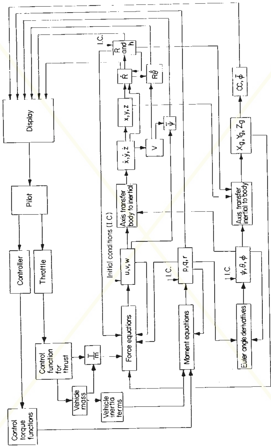
Figure 1.- Block diagram of equations showing information flow of computer program.
