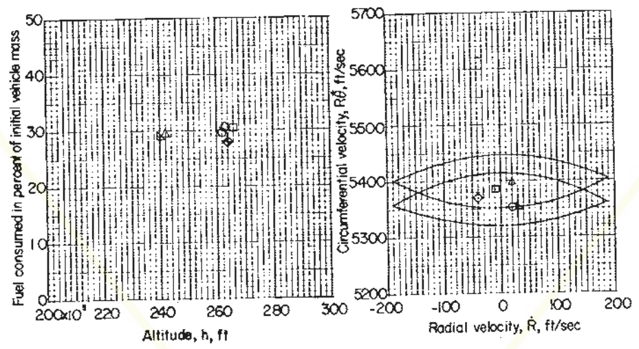
(a) Flights initiated at an altitude of 1 \times 10^6 feet, R\theta nominal (7,575 ft/sec), and rate of descent 200 ft/sec greater than nominal value ( \dot{R} = -3,067 ft/sec).
