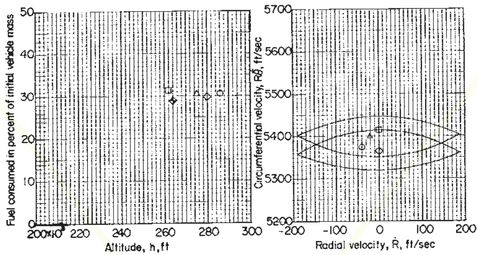
(c) Flight initiated at an altitude of 1 \times 10^6 feet, \dot{R} nominal ( \dot{R} = -2,867 ft/sec), and R\dot{\theta} = 200 ft/sec greater than nominal value (7,775 ft/sec).
